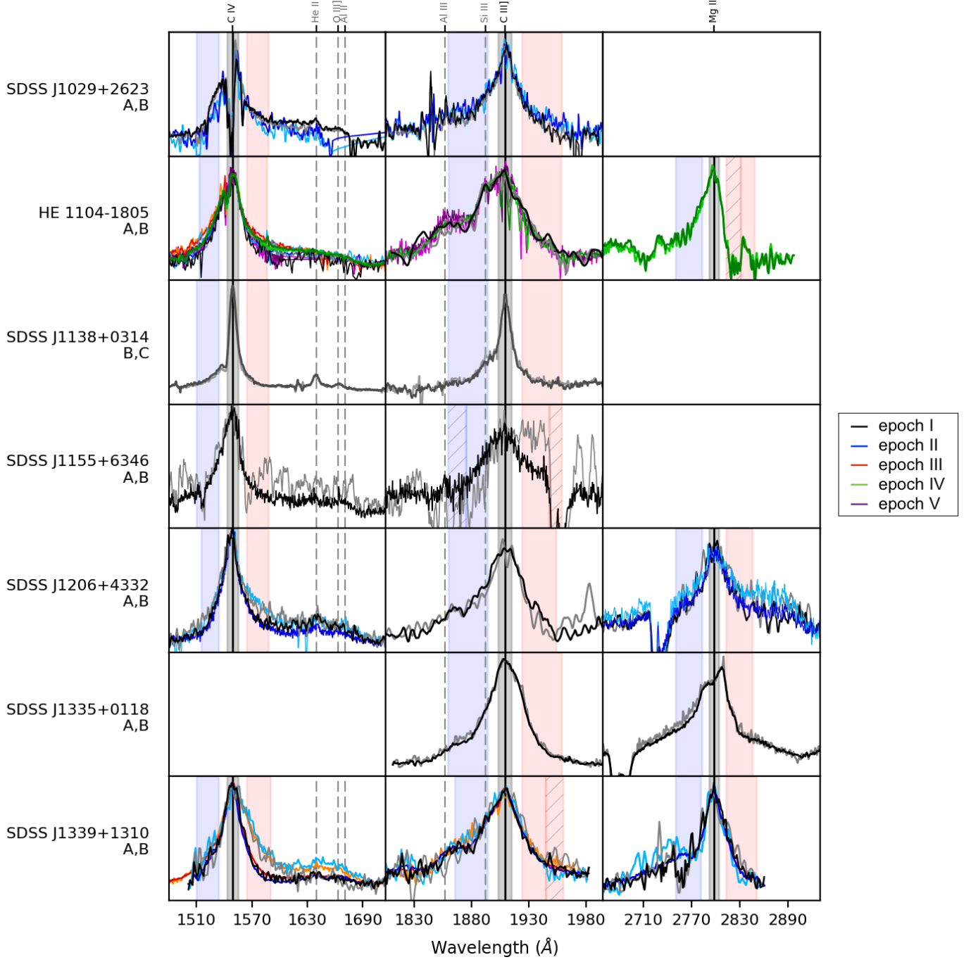
Fig. 3. Continuation of Figure 1.
