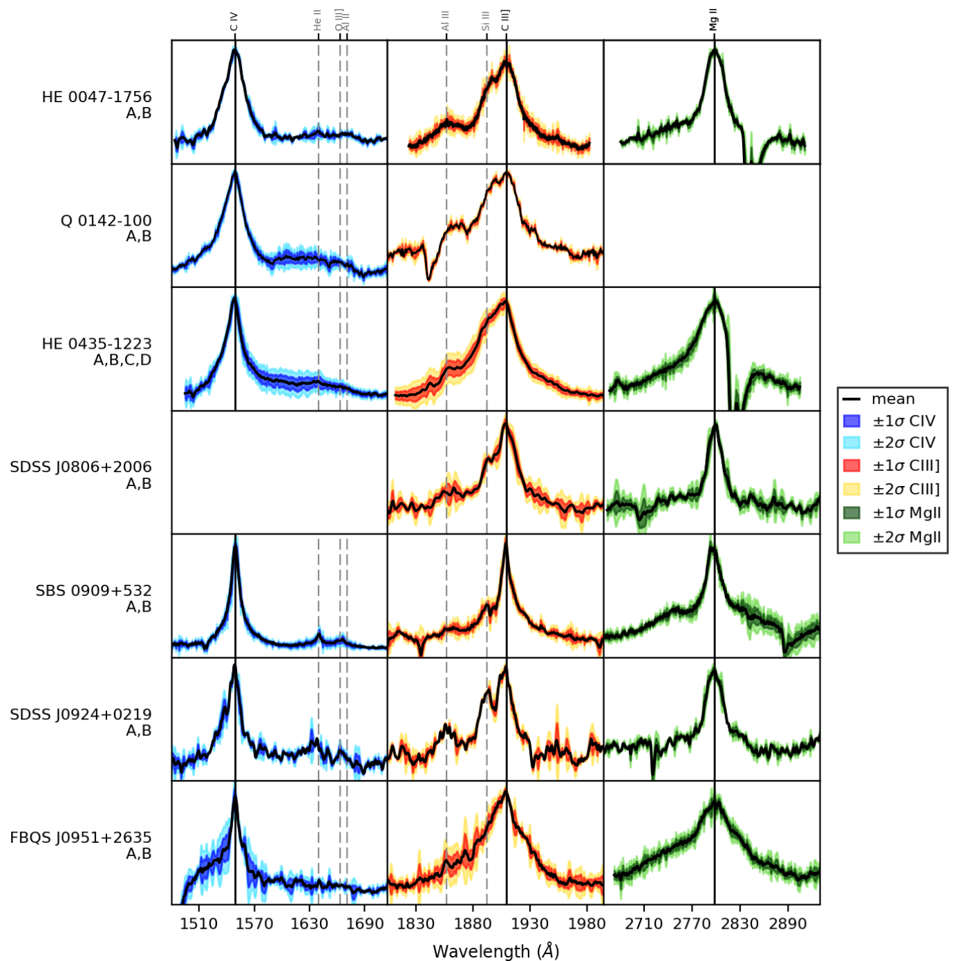
Fig. 5. Average (black) spectra for the C IV, C III], and Mg II emission lines with one (dark blue, red, and green) and two (light blue, red, and green) sigma intervals. We did not take into account noisy spectra and spectra that show absorption features in the line core (as in the case of Mg II in SDSS J1004+4112). The y-axis is in arbitrary units of flux.
