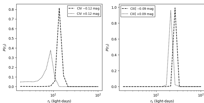
Fig. 10. Joint likelihood for C IV (left panel) and C III] (right panel) after subtracting (dashed lines) and adding (dotted lines) the average impact of microlensing of the corresponding core.
