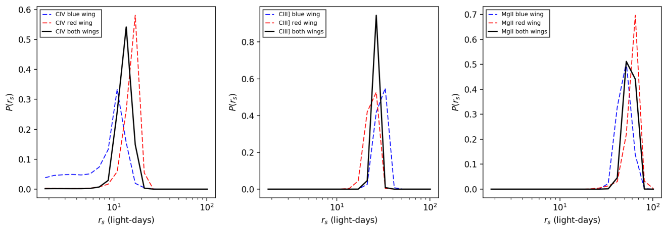
Fig. 9. Joint likelihood (solid black line) for C IV (left panel), C III] (middle panel), and Mg II (right panel). Dashed lines show the Joint likelihood functions for the red and blue wing, respectively.
