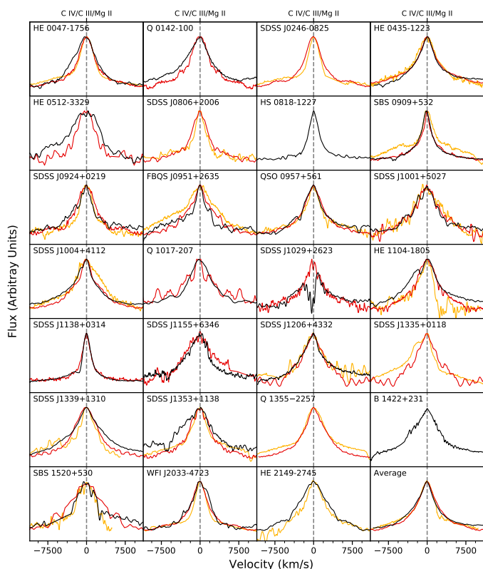
Fig. 12. Line profiles of C IV (black), C III] (red), and Mg II (yellow) as a function of velocity.
