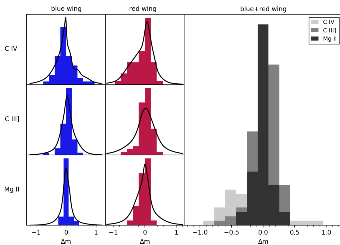
Fig. 7. Histograms of microlensing magnification difference between image pairs (in the same epoch) in the blue and red wings of C IV, C III], and Mg II. Black curves show the corresponding Gaussian kernel density estimates of the PDFs.
