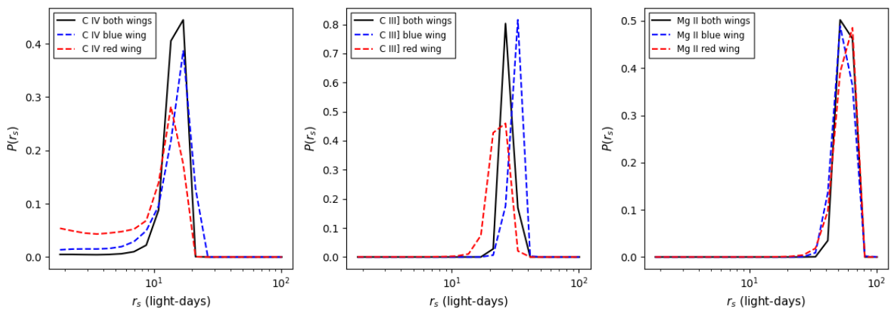
Fig. 11. Joint likelihood (solid black line) for C IV (left panel), C III] (middle panel), and Mg II (right panel) for "pure" microlensing signals (see Section 4.3). Dashed lines show the joint likelihood functions for the red and blue wing, respectively.
