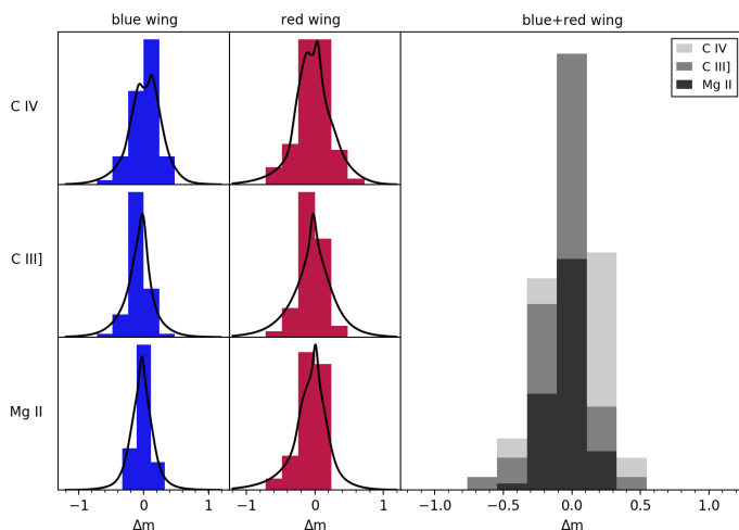
Fig. 8. Histograms of magnitude difference for the same image at different epochs in the blue and red wings of C IV, C III], and Mg II. Black curves show the corresponding Gaussian kernel density estimates of the PDFs.
