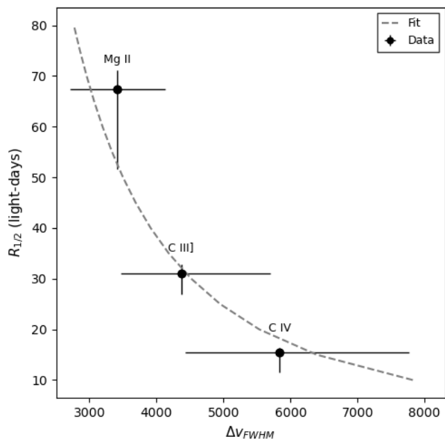
Fig. 14. Average emission region size as a function of the line broadening for C IV, C III], and Mg II. The line of best fit according to Eq. 5 is shown as a dashed gray line.
