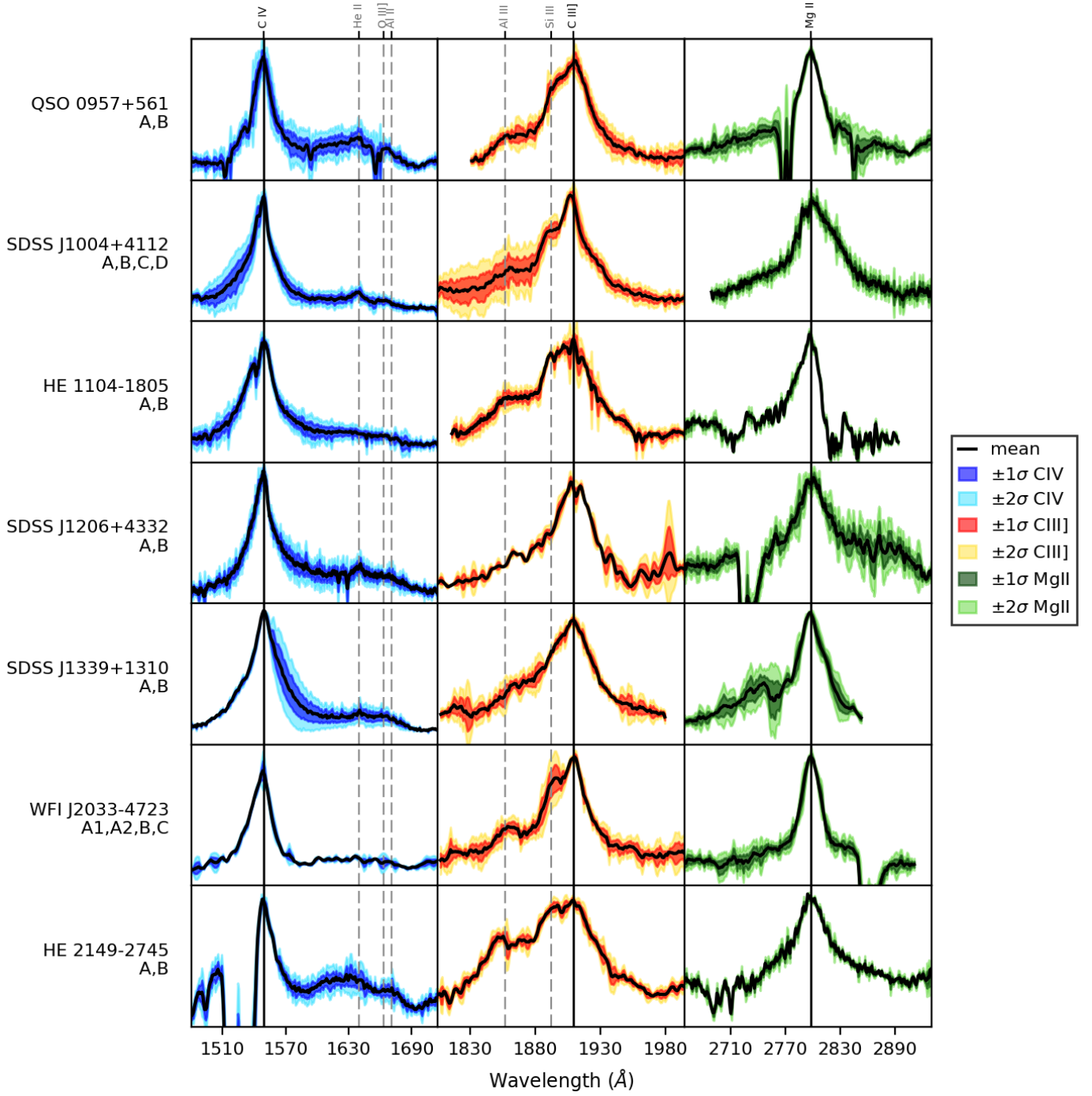
Fig. 6. Continuation of Figure 6.
