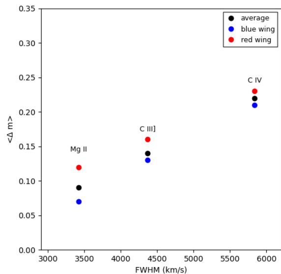
Fig. 13. Average amplitude of microlensing between images as a function of the line broadening for C IV, C III], and Mg II.
